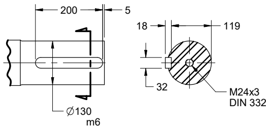
SHAFT DETAIL
